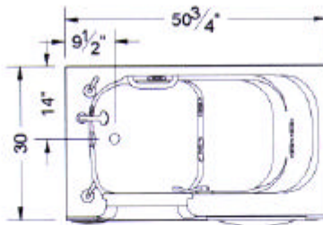
TOP VIEW - SCALE \frac{3}{8}'' = 1'-0''
