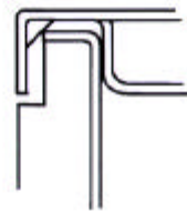
Assembly Joint Detail side-to-backwall DETAIL A
