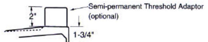
Cross Section Threshold A-A
